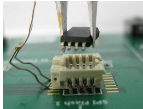
2) Remove the Serial Flash from the Engineering socket
