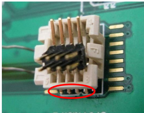
4) Slide the SMT connector between the socket contact pins and the plastic so that connector pins are shifted outside the socket then you can insert the other side.
