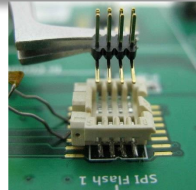
3) Insert the DediProg Special SMT connector
